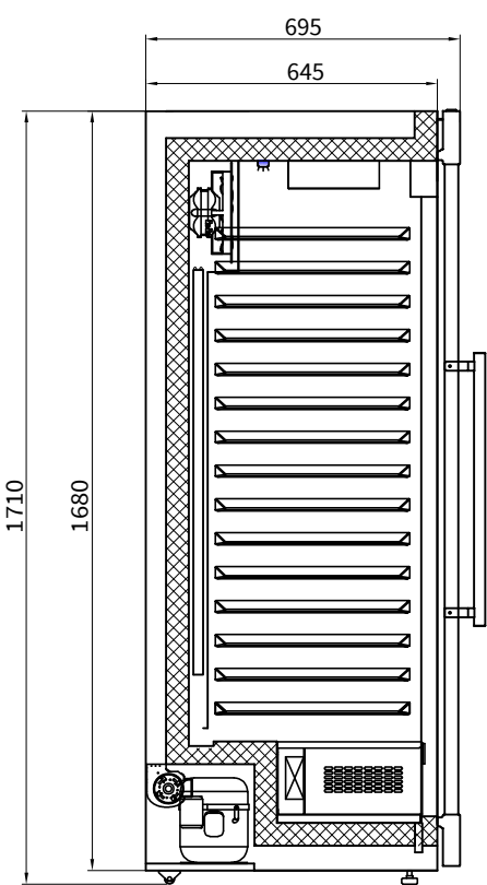
SIDE VIEW
