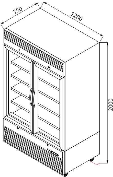
ISOMETRIC
