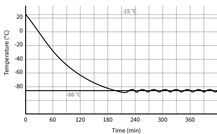
PULL DOWN TIMES
