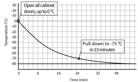
PERFECT RECOVERY TIME
