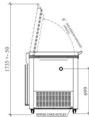
4 SIDE VIEW
