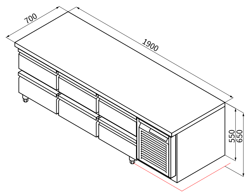
ISOMETRIC
