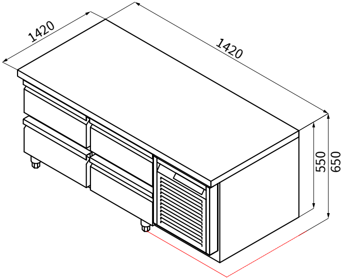
ISOMETRIC
