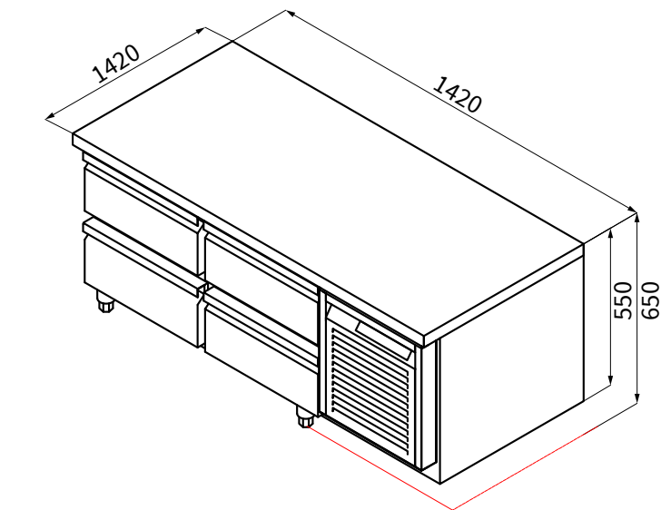
ISOMETRIC
