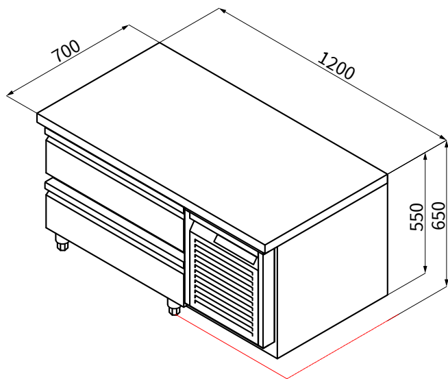
ISOMETRIC
